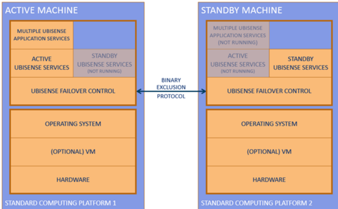
A two machine setup running a Ubisense system. At any one time, one machine is in the active state, and the other machine is in the standby state.
